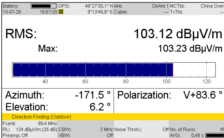
The final meters of direction finding: Looking for the maximum level.
