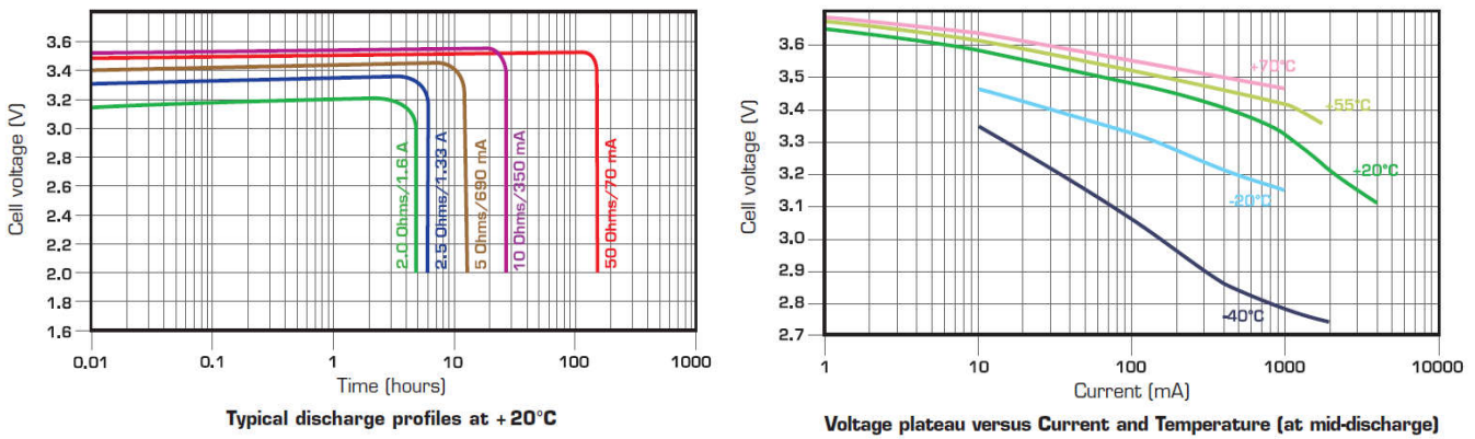
Fig. 1 - LSH 20 primary lithium battery graphs
