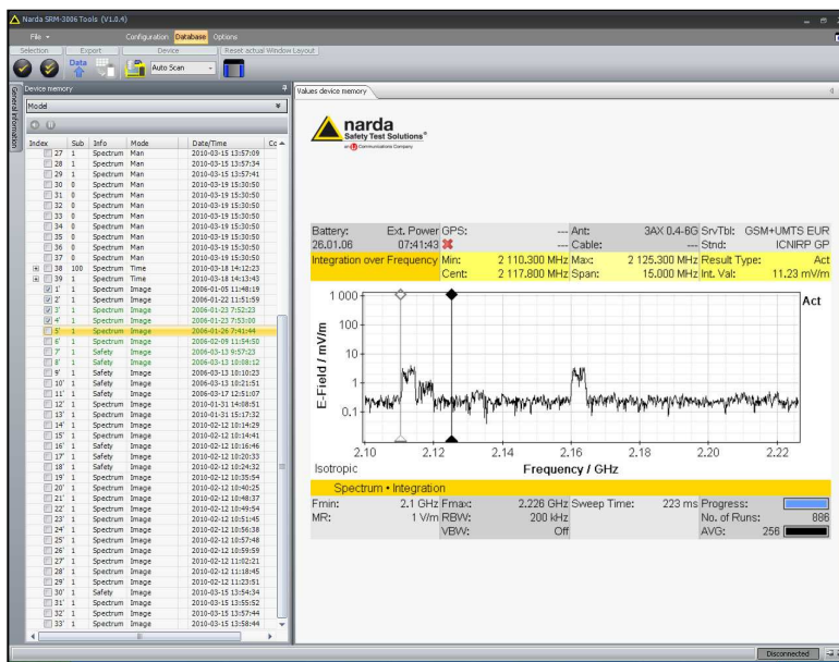
Figure 1: Example screenshot. The screenshot function can be used to insert measurement results directly into test reports, showing numerical values and graphical representations at a glance. Screenshots can also be attached to e-mails for distribution and discussion.
