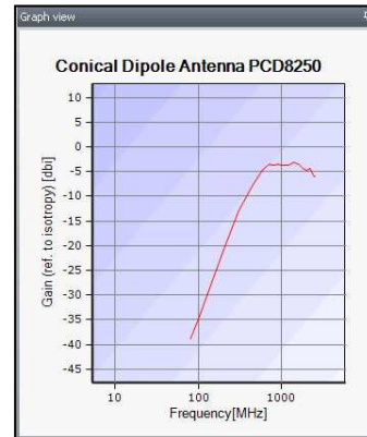
Figure 2: Graphical display of antenna factors. These can be directly edited using the PC software.
