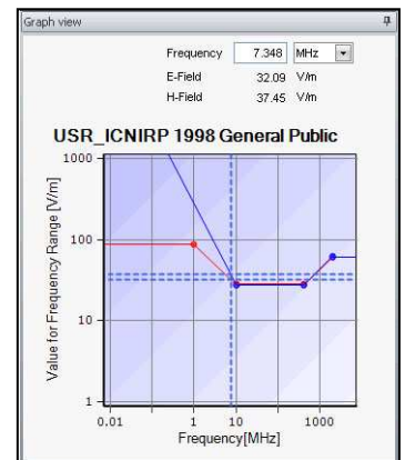
Figure 3: Graphical display of limit value curves for a standard.
