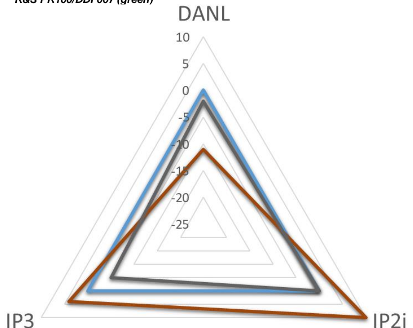
Figure 25: Specification of R&S EB500 low distortion mode (brown), normal mode (gray)
