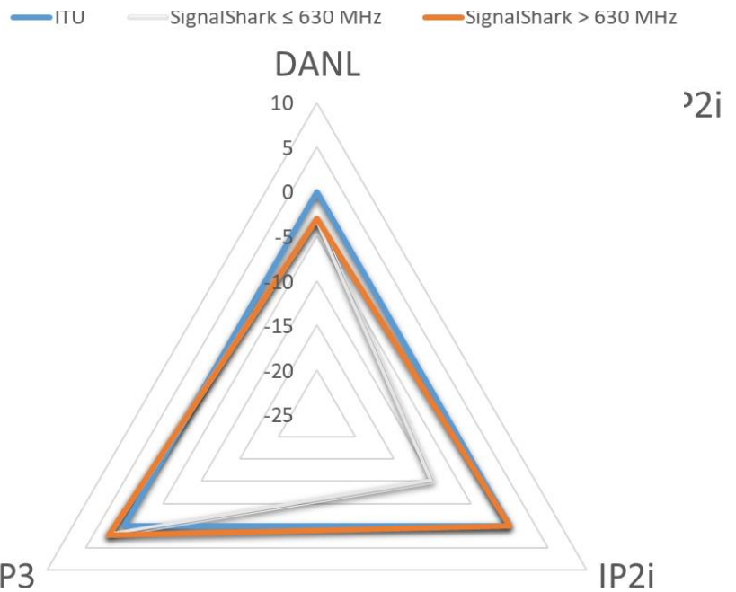
Figure 23: SignalShark dynamic range parameters compared with the ITU recommendations
