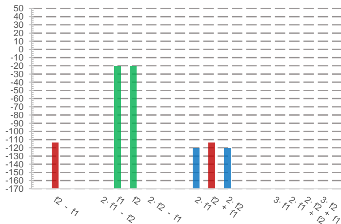
Figure 8: SignalShark dynamic range for -20 dBm signals at 890 MHz and 2150 MHz
