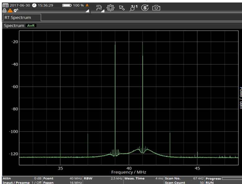
Figure 1: Narda SignalShark
