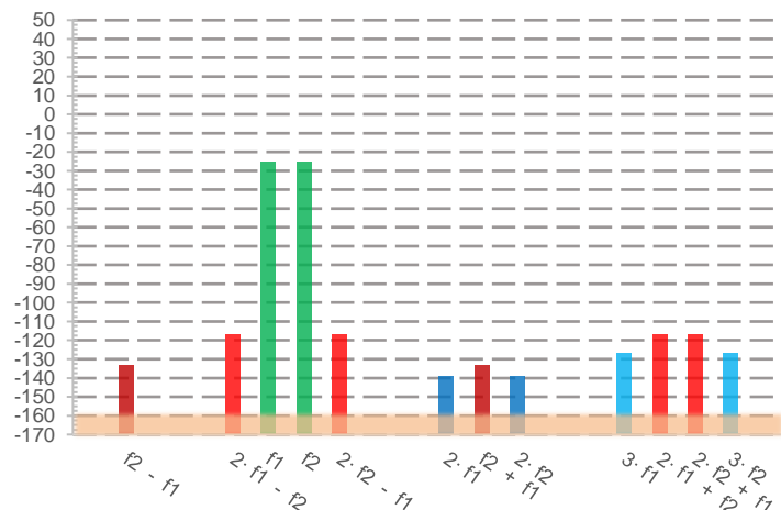
Figure 7: SignalShark dynamic range for -25 dBm signals at 19 MHz and 20 MHz
