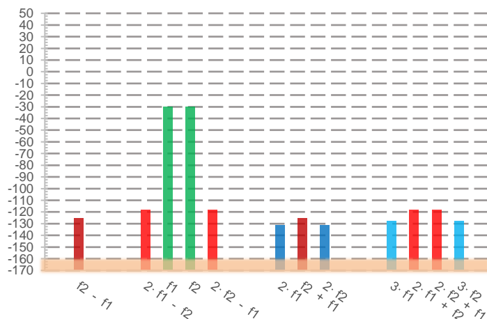
Figure 9: SignalShark dynamic range for -30 dBm signals at 928 MHz and 929 MHz
