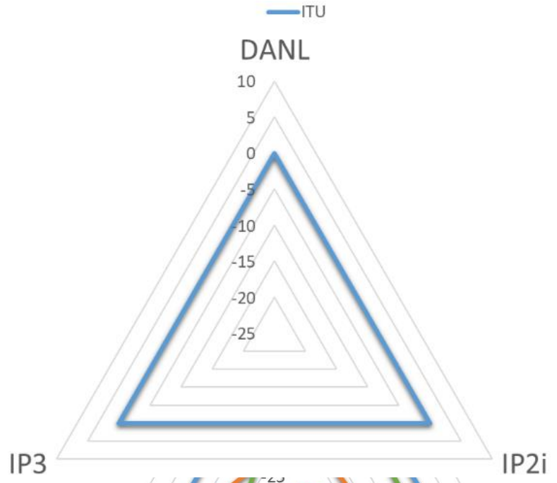
Figure 2: ITU recommended dynamic range parameters as a relative graph
