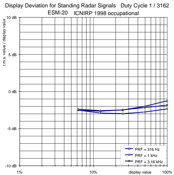
Figures A7-A12: Deviation of RMS value from display value for RadMan (ESM-20)
