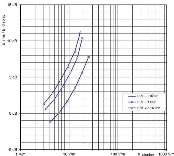
Figures A1-A6: Deviation of RMS value from display value E-field probe EF1891
