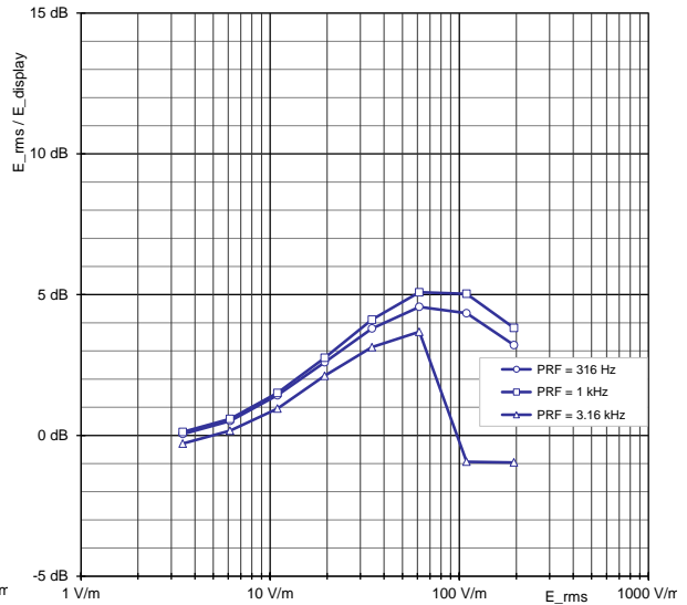
Display Deviation for Standing Radar Signals Duty Cycle 1 / 1000 for E-Field Probe EF1891
