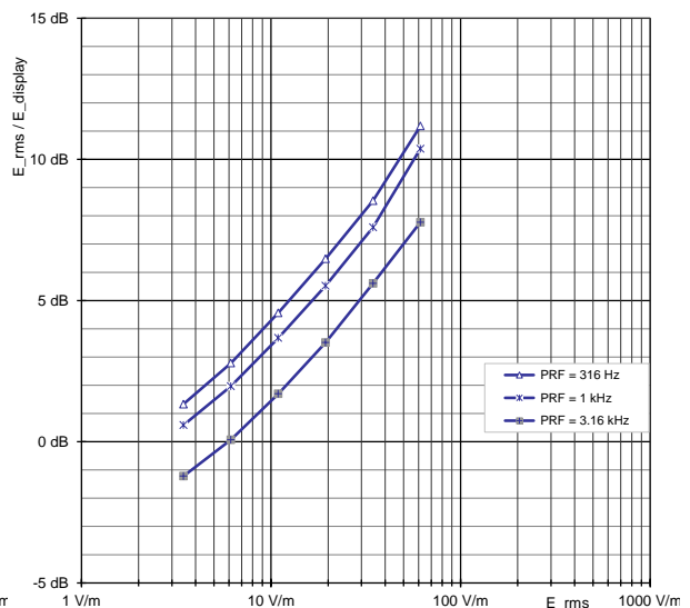
Figures A1-A6: Deviation of RMS value from display value E-field probe EF1891
