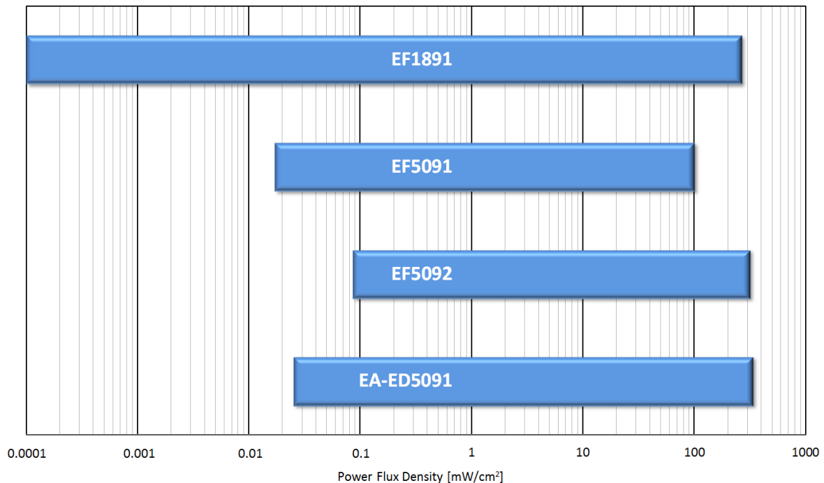
Figure 3: Dynamic ranges of thermocouple and diode probes
