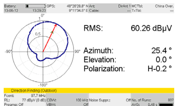
Figure 2 – Bearing 1: Ideal situation for a horizontal scan. The polar diagram shows the directional characteristic of the direction finding antenna because the field is undistorted (compare Figure 9). Interpretation is simple, the bearing of the source is easily found.
