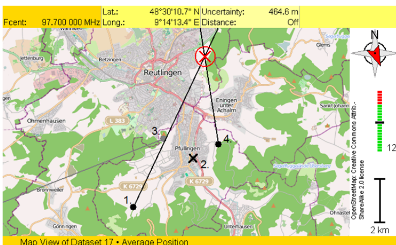
Figure 8: The instrument displays the bearing result of the saved horizontal scan on the map directly on site. False bearing 2 was rejected, and false bearing 3 points in the wrong direction because of shadowing by the hill. The two successful bearings 1 and 4 are enough to pinpoint the location of the transmitter.
