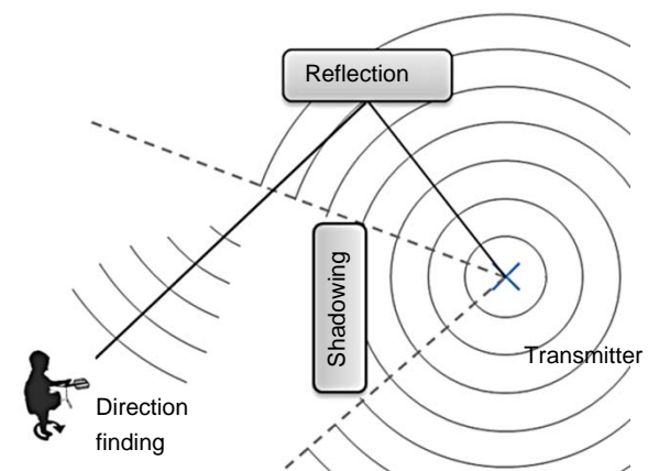
Figure 4: Shadowing and reflection during direction finding.
