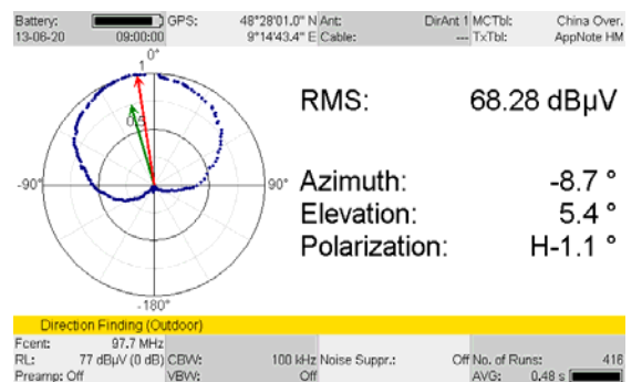
Figure 7 – Bearing 4: Ideal conditions just like Bearing 1 (Figure 2).
