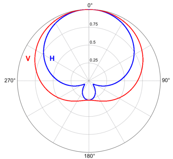
Figure 9: The typical directional characteristic of Directional Antenna 1 at 150 MHz for vertical (V) and horizontal polarization (H).
