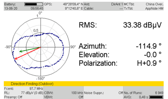
Figure 6 – Bearing 3: Horizontal scan from an unfavorable location behind a hill. Shadowing and reflections cause the direction to be determined incorrectly. An expert can see from the shape of the measured characteristic that the measurement is incorrect.
