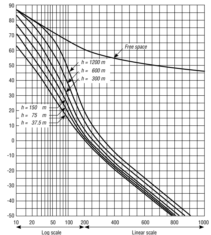
Figure 4: Field strengths for 1 kW radiated power (ERP) as a function of the height of the transmitting antenna h ; receiving antenna height = 10 m; unevenness in terrain = 50 m; frequency range 30–250 MHz. Source: ITU-R Recommendation P.370-7 [4]
