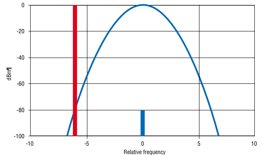
Figure 1: Example of spurious reception
